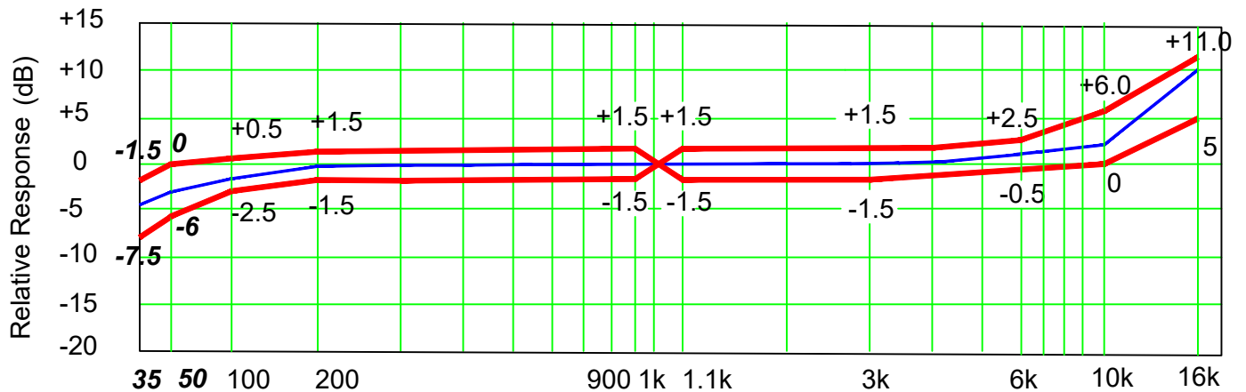
Typical Free Field Response Normalized to 1kHz Standard Mode
