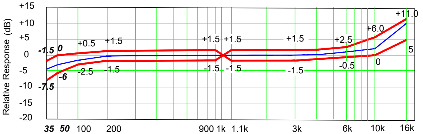
Typical Free Field Response Normalized to 1kHz Low Power Mode
